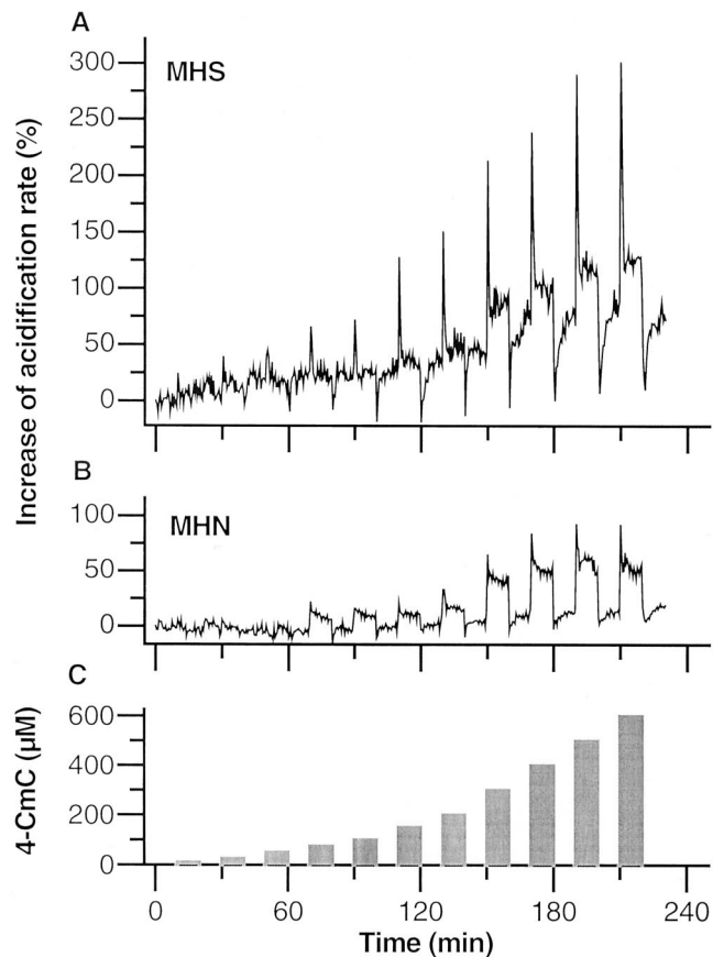
Fig. 2. Acidification responses at increasing 4-chloro- m -cresol (4-CmC) concentrations. (A) Normalized increase in proton secretion rate recorded from a malignant hyperthermia-susceptible (MHS) culture. (B) Rate recordings from a malignant hyperthermia-normal (MHN) culture. (C) Concentrations of 4-CmC applied in the test.
